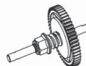
T4971/24 Kit Slipper
