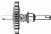
T4971/14 Slipper Set
