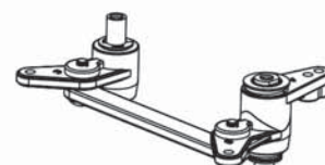
T4972/16 Sauve servo
