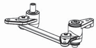
T4972/16 Servo Saver
