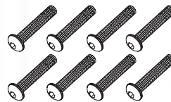
FTX-SBH053 Umbrella head hex screw M3x25
