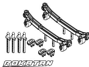
FTX10155 Complete Body Mount Set
