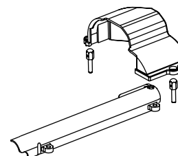
FTX10115 gear box cover
