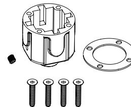
FTX10103 differential case
