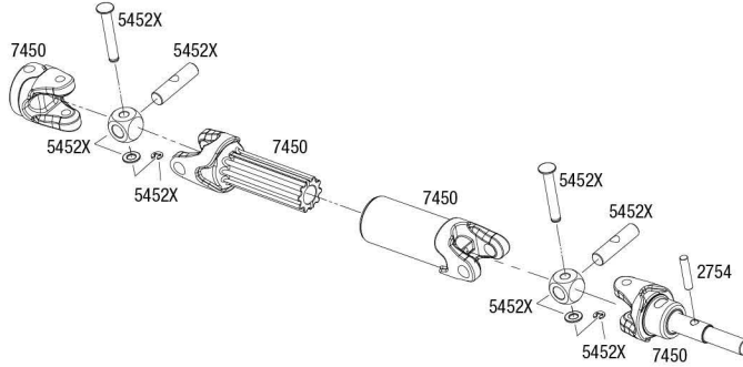
Front Driveshaft Assembly
