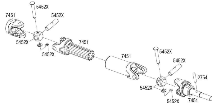
Rear Driveshaft Assembly
